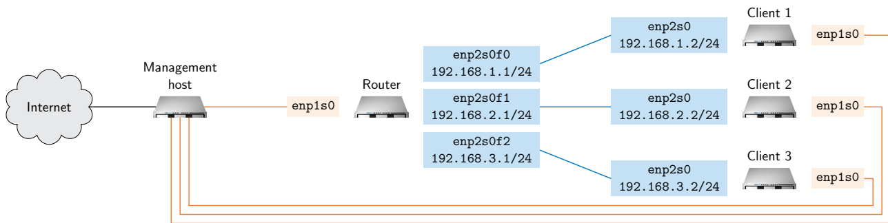
Figure 1: Testbed with management host, clients and router
